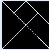
Convex Polygon 1
